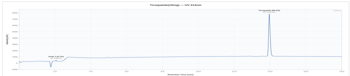
Tirzepatide 10mg - AP-TZ10-0726: UV Chromatogram
