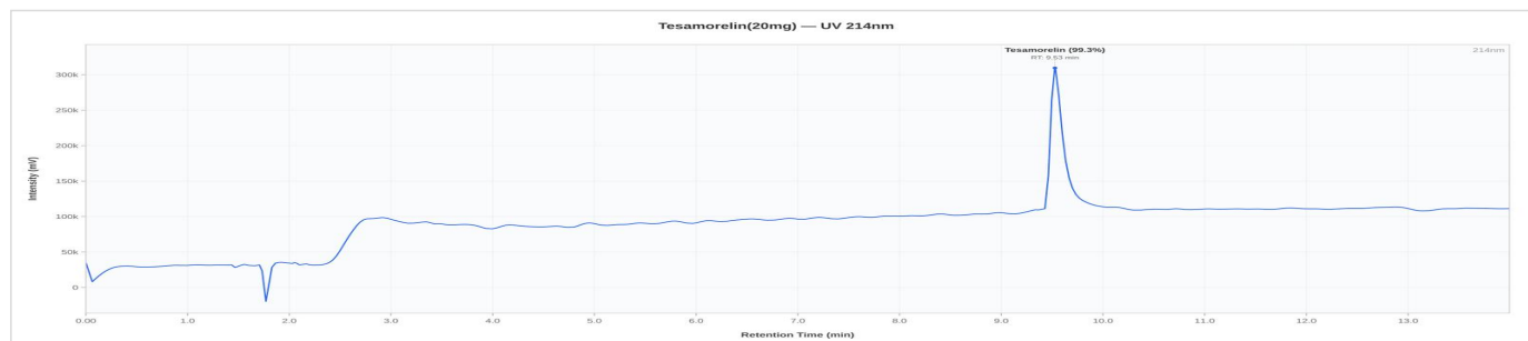
Tesamorelin 20mg - AP-TS20-0726: UV Chromatogram
