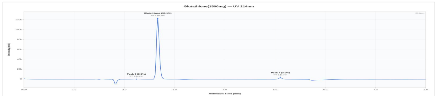
Glutathione 1500mg - AP-GLU15-0726: UV Chromatogram
