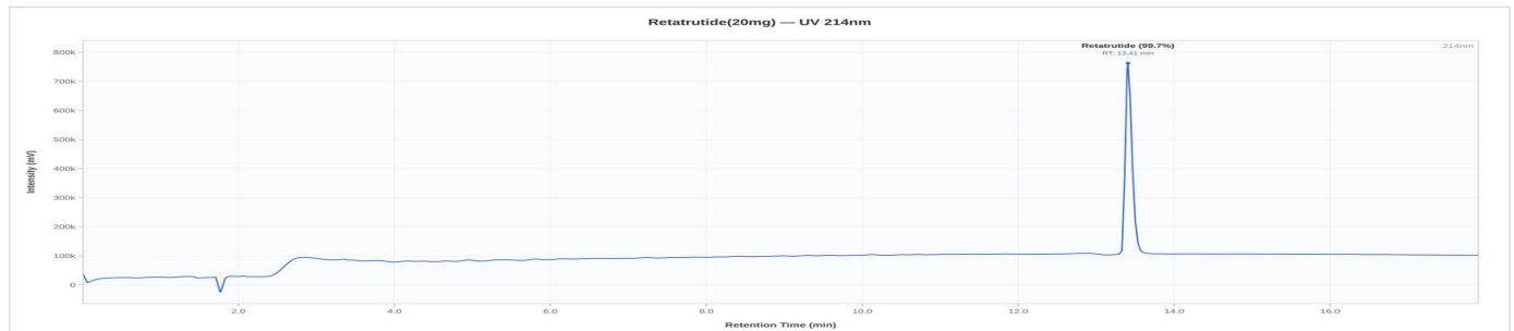
AP-3RT 20mg - AP-RT60-0726: UV Chromatogram
