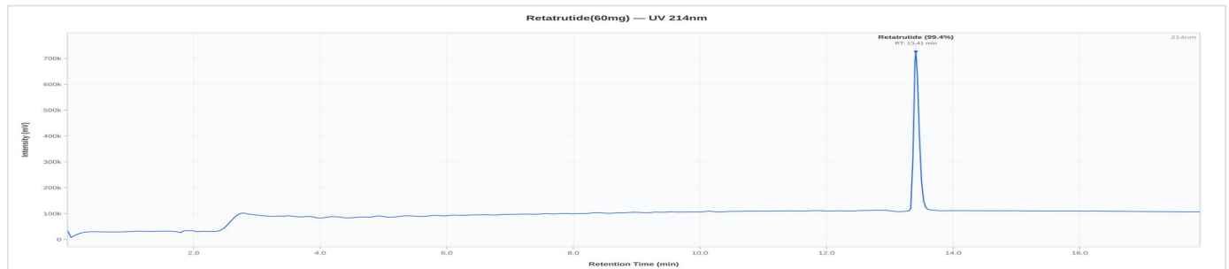
AP-3RT 60mg - AP-RT60-0726: UV Chromatogram
